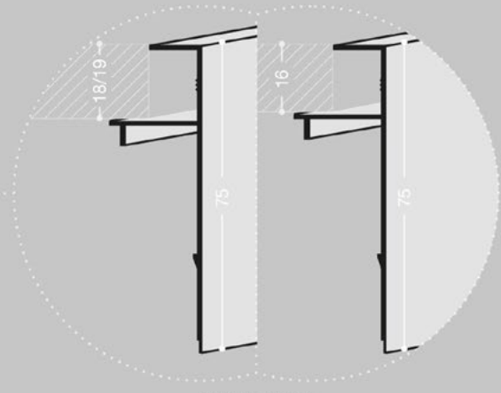
PROFIL OBEN cod. FBS7518 ( Platten 18 - 19 mm ) cod. FBS7515 ( Platten 16 mm )
